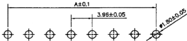
RECOMMENDED P.C.B LAYOUT(TOP VIEW) TOLERANCES: ±0.10mm
